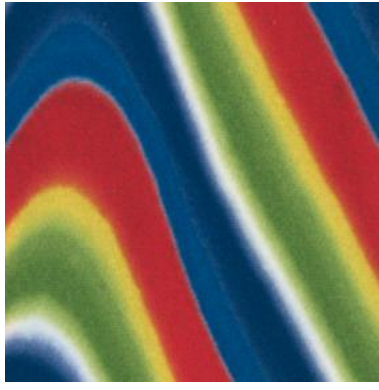
TORNADO
